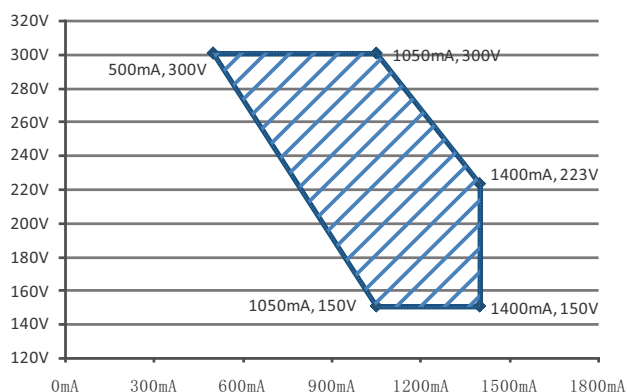
◎ XLG-320-H
