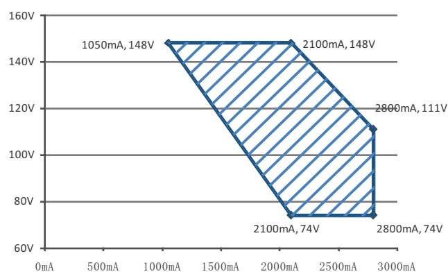
◎ XLG-320-V
