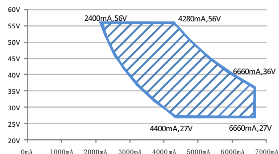
◎ XLG-240-H-DA2
