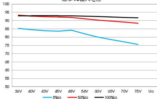
VCF4812EBO-120W(F)R3-N 效率VS输入电压
