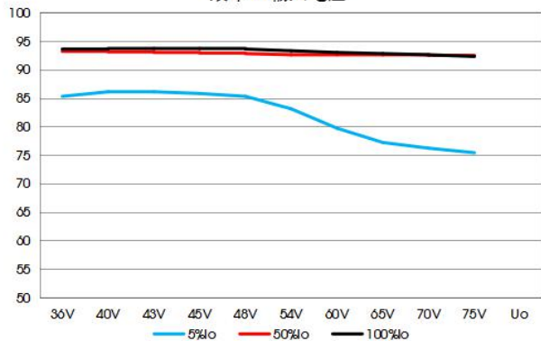
VCF4812EBO-120W(F)R3-N 效率VS输入电压
