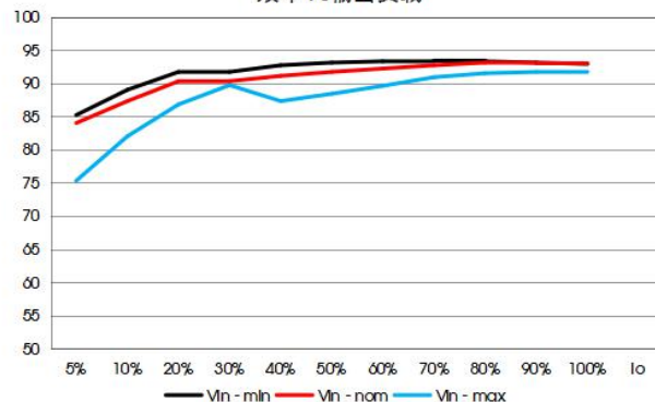
VCF4805EBO-120W(F)R3-N 效率VS输出负载
