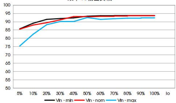
VCF4812EBO-120W(F)R3-N 效率VS输出负载
