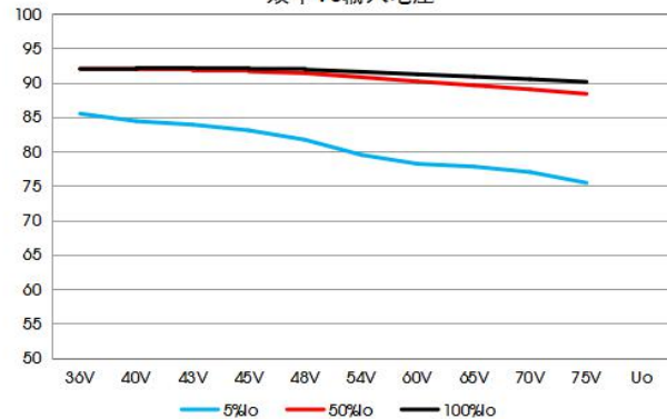
VCF4824EBO-120W(F)R3-N 效率VS输入电压
