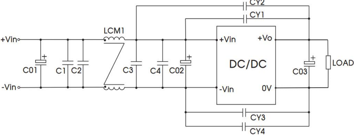
VCF4824EBO-100W(F)R3-N
