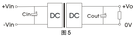
VCF4803/05/12EBO-100W(F)R3-N
