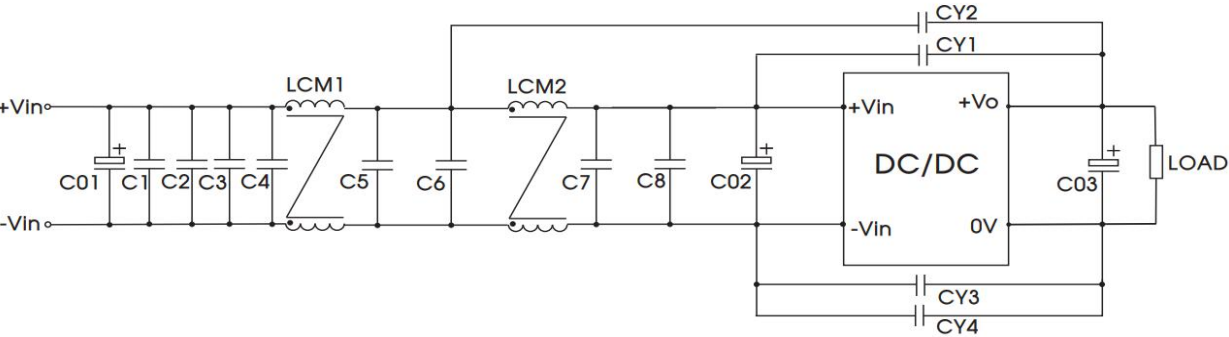
VCF4824EBO-100W(F)R3-N
