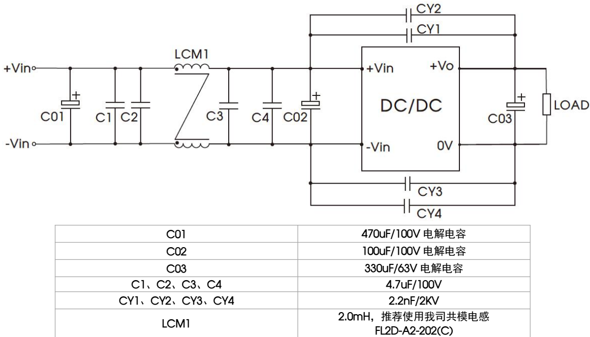
VCF4803/05/12EBO-100W(F)R3-N
