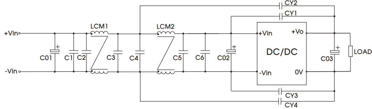
VCF4803/05/12EBO-100W(F)R3-N
